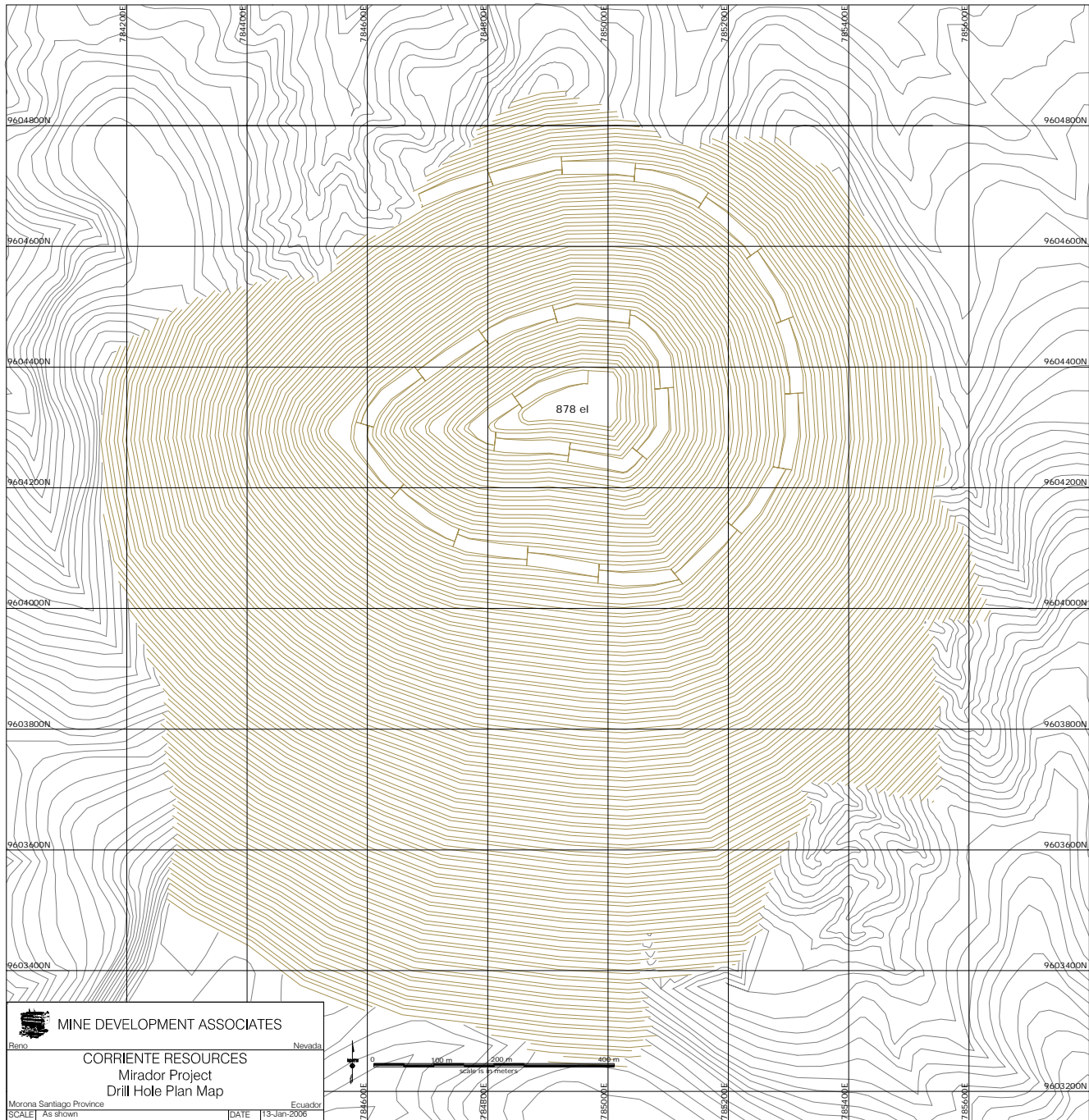
Figure 17.6 Ultimate Designed Pit
